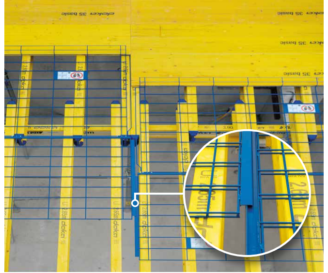
Safeflex sliding mesh with guide rail
