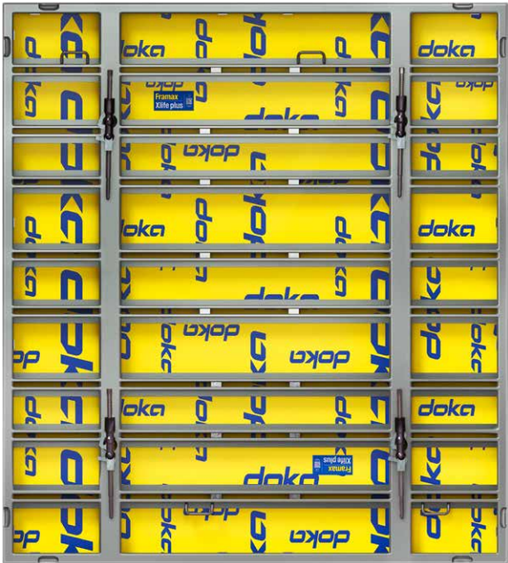
Framax Xlife plus 2.70 x 3.00 m: only four form ties for 8.1 m 2 of formwork
