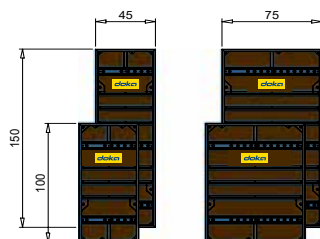
Universal panels for columns with 5 cm grid
