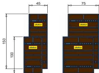
Universal panels for columns with 5 cm grid
